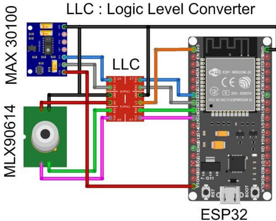
Fig. 4. It shows the diagram circuit of the proposed system
