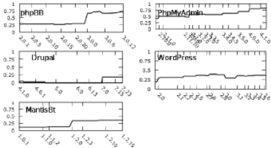
Fig. 5. Methods ratio over total number of functions and methods
