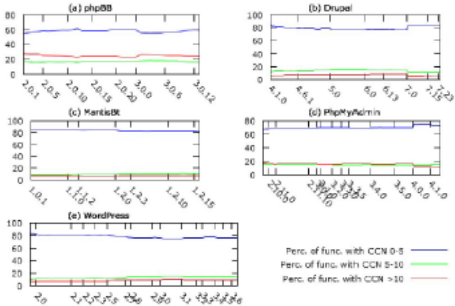
Fig. 4. Evolution of functions in three complexity ranges over time
