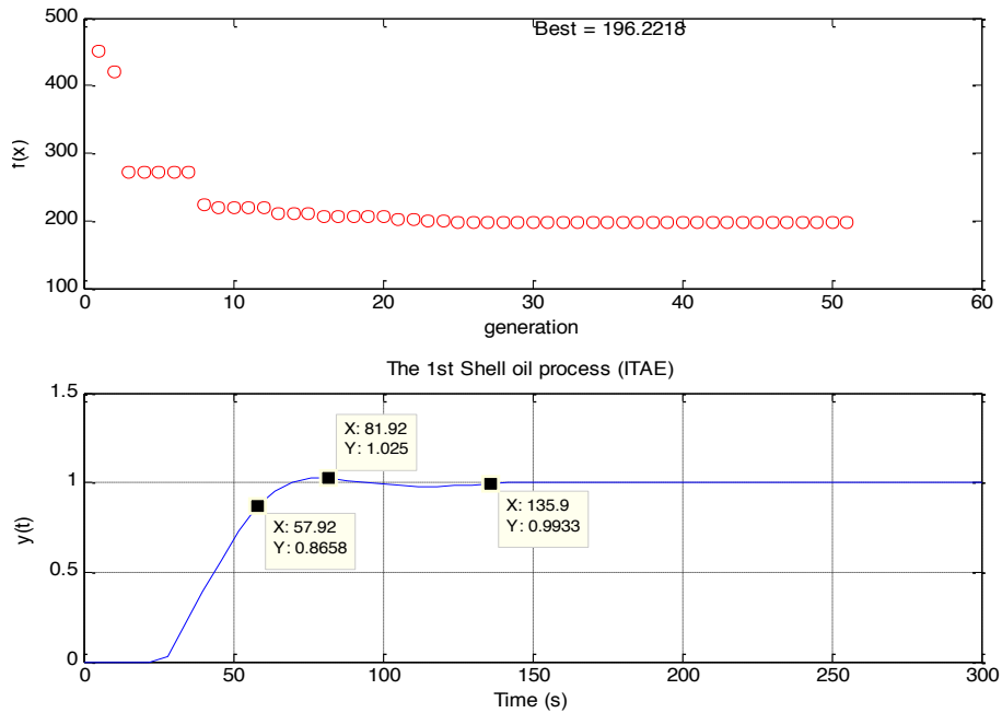
Fig. 3. the GAs process with ITAE objective function.
