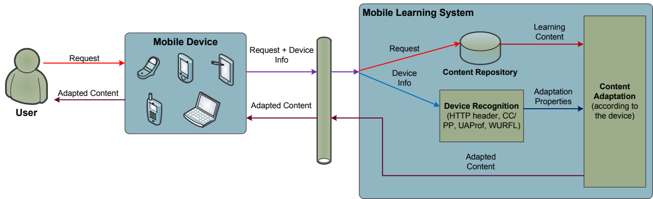
Figure 1. Scheme of a device feature recognition module integrated in an m-Learning system.
