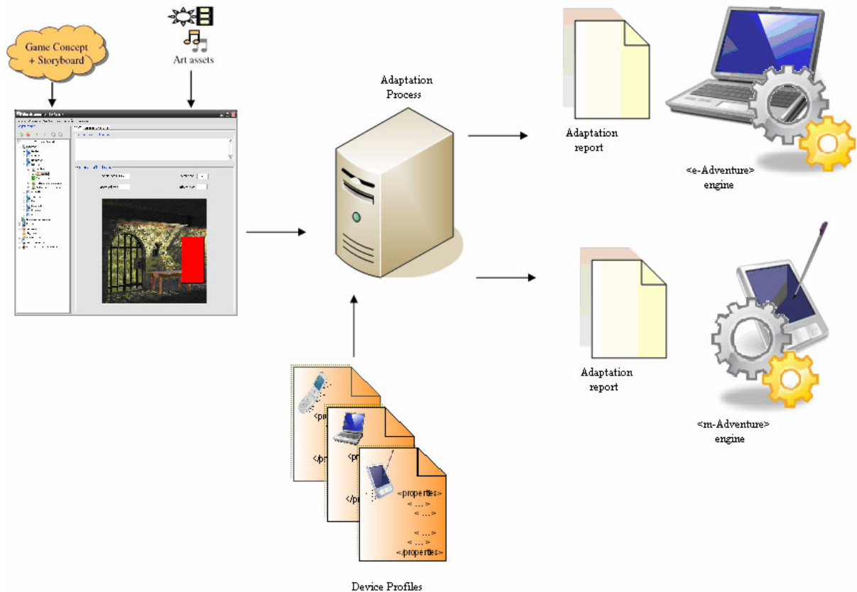
Figure 5. Scheme of the exportation procedure in <e-Adventure>
