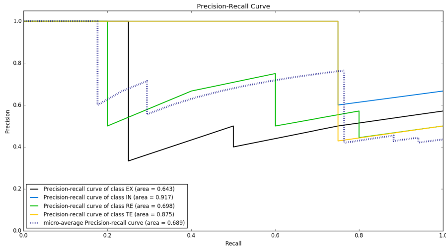
Fig. 4. Precision-Recall Curve
