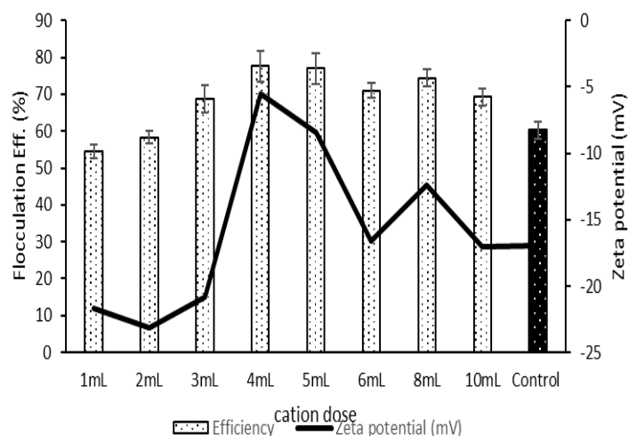
Fig. 2. Effect of K + on bioflocculation efficiency of A. flavus bioflocculant produced from chicken viscera hydrolysate
