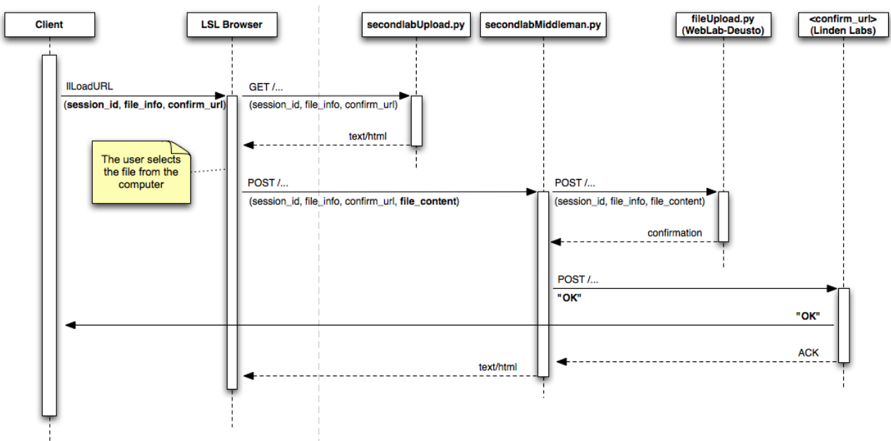
Figure 8. The web-uploader sequence
