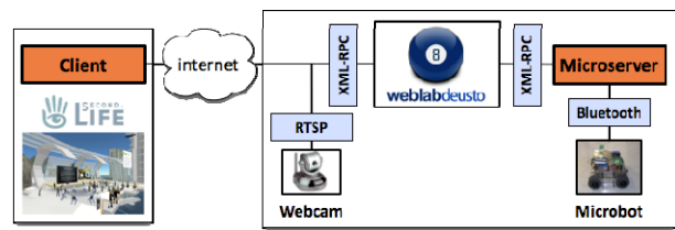
Figure 7. Architecture of SecondLab
