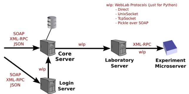
Figure 3. WebLab-Deusto servers
