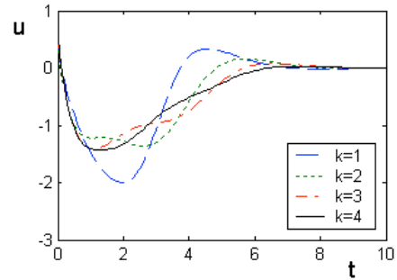
Figure 2. Curves for control law when k = 1, 2, 3, 4
