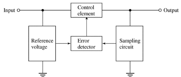
Figure 2. Voltage controller
